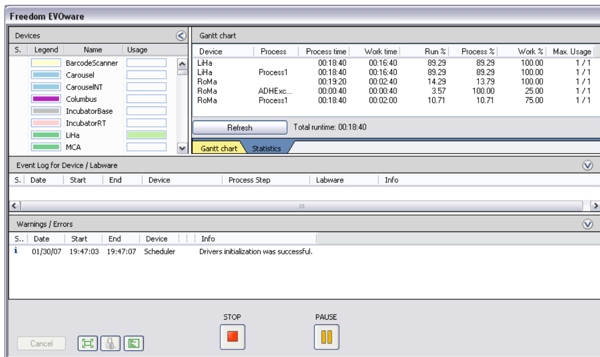
Fig. 12-8 Process runtime - Extended view (showing the Statistics window)
